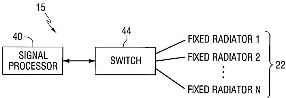
FIG. 2 PRIOR ART
